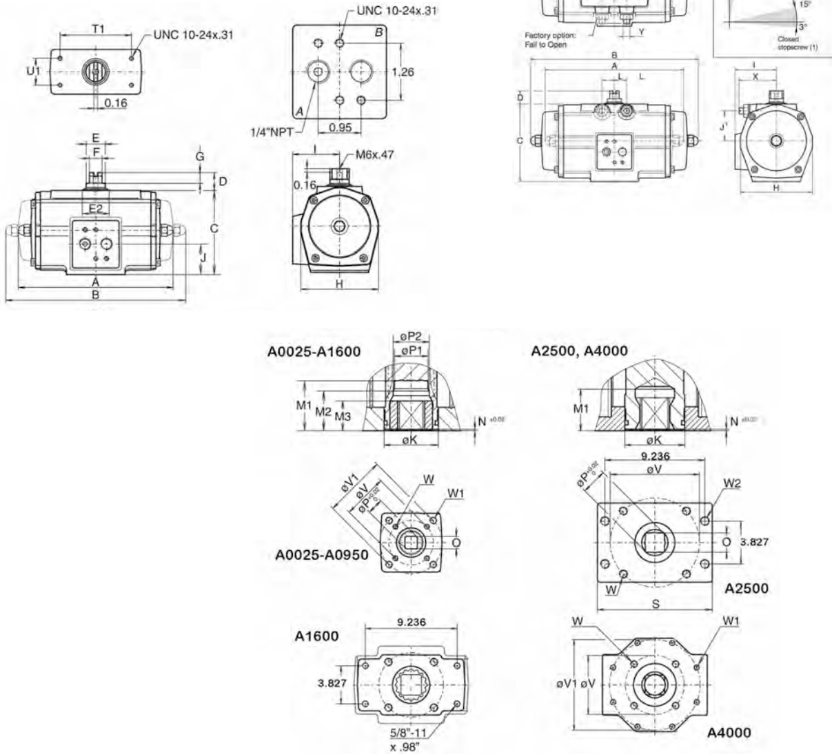
Rack & Pinion Actuator Envelop Dimensions
