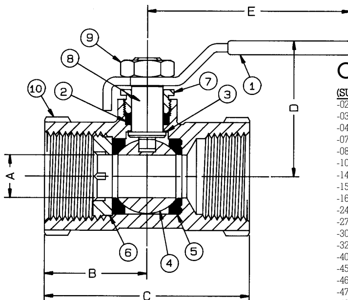
CARBON STEEL UNI-BODY SATURN® BALL VALVE
