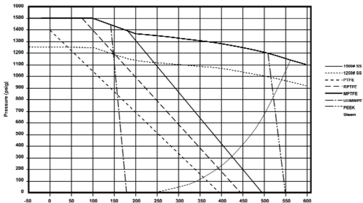
1500# SS P-T Rating (Graph 12)
