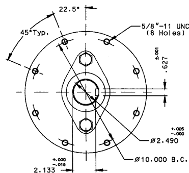
ACTUATOR MOUNTING: 10" & 12"
