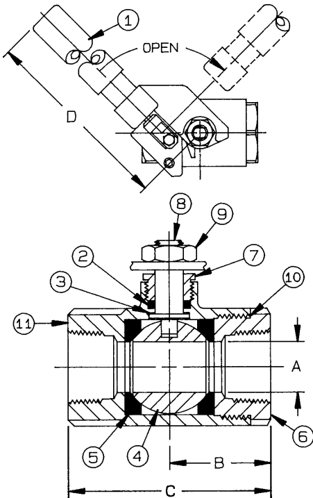
BRONZE BALL VALVE WITH SPRING RETURN HANDLE
