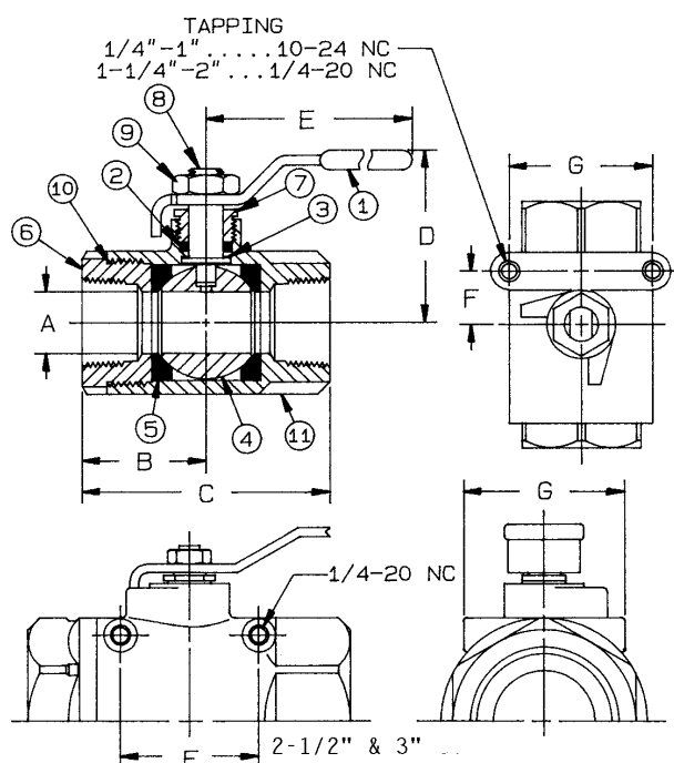
CARBON STEEL BALL VALVE
